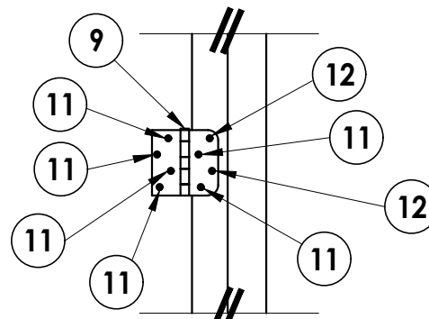
HINGE DETAIL
