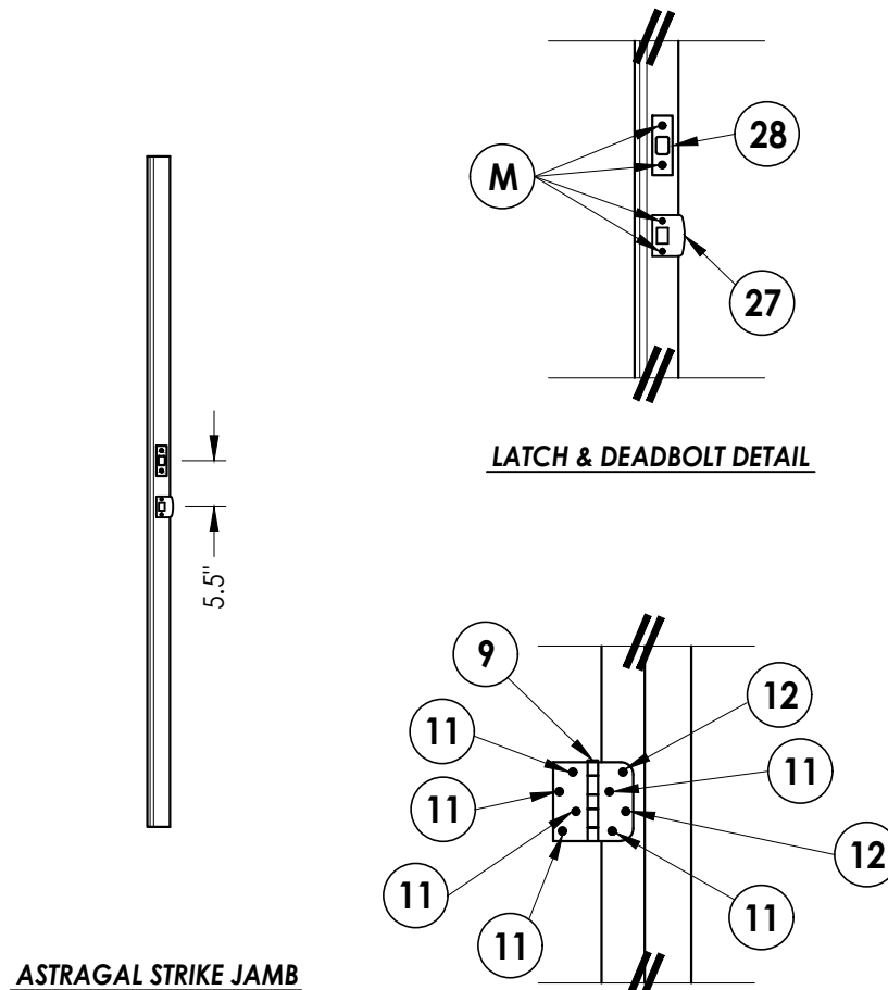
ASTRAGAL STRIKE JAMB
